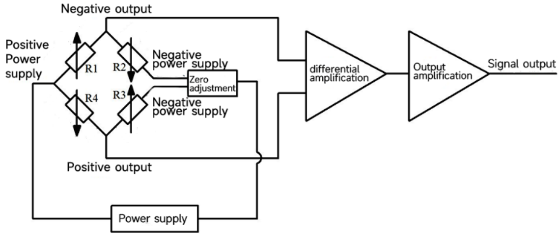
Picture 2.1 pressure sensor schematic
